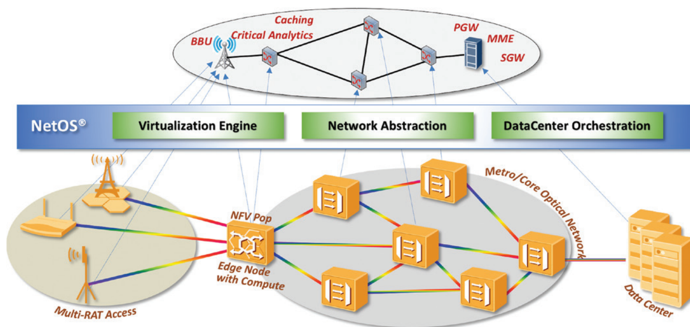
Figure 1 – NetOS® Topology Abstractions – Virtual overlay over infrastructure underlay
